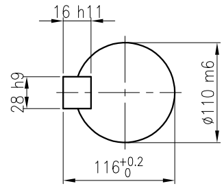
OUTPUT SHAFT (28 x 16 x 187)
