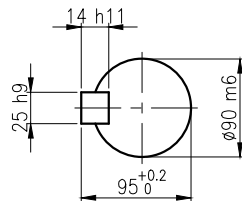
OUTPUT SHAFT (25 x 14 x 144)
