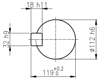
OUTPUT SHAFT KEY 32 x 18 x 155
