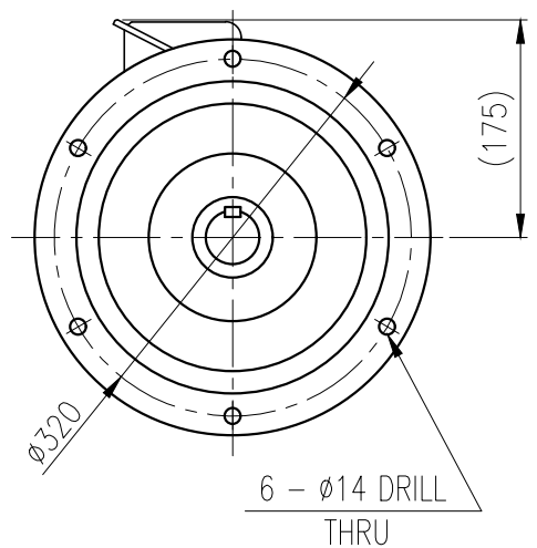
VIEW "Q"
