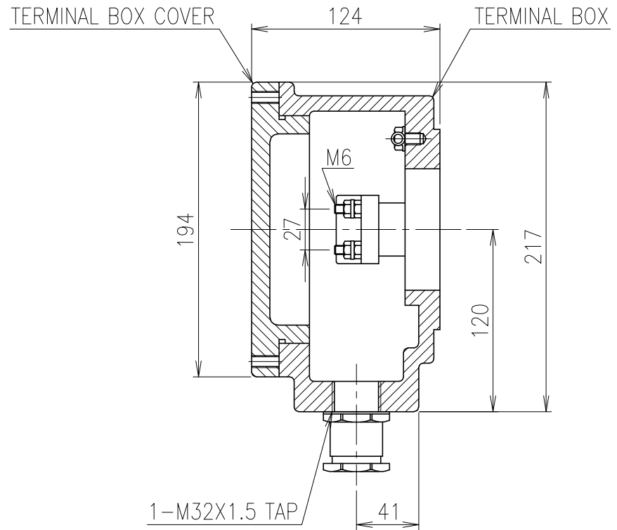
SEC. A-A'
