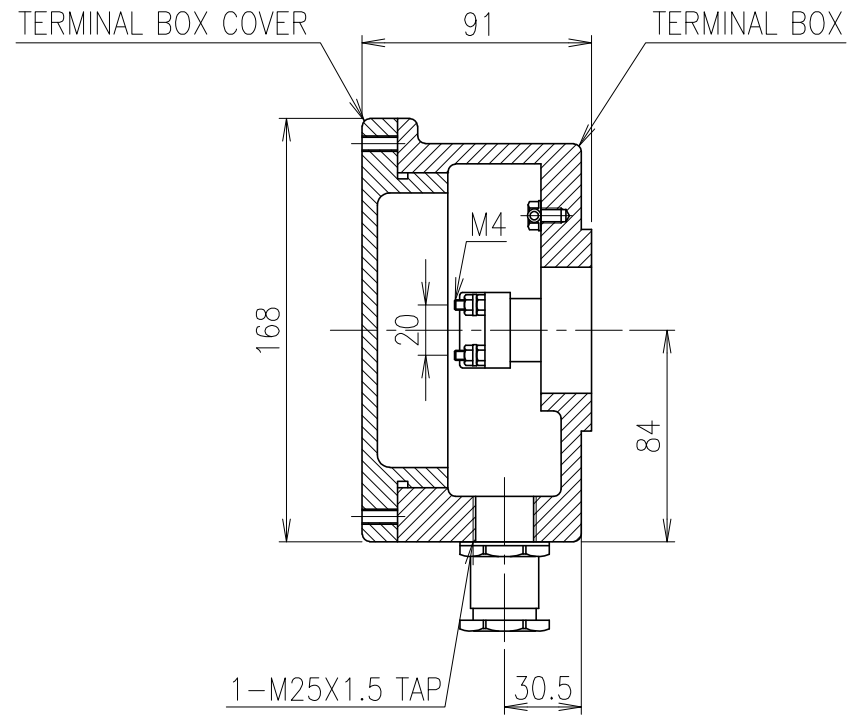
SEC. A-A'
