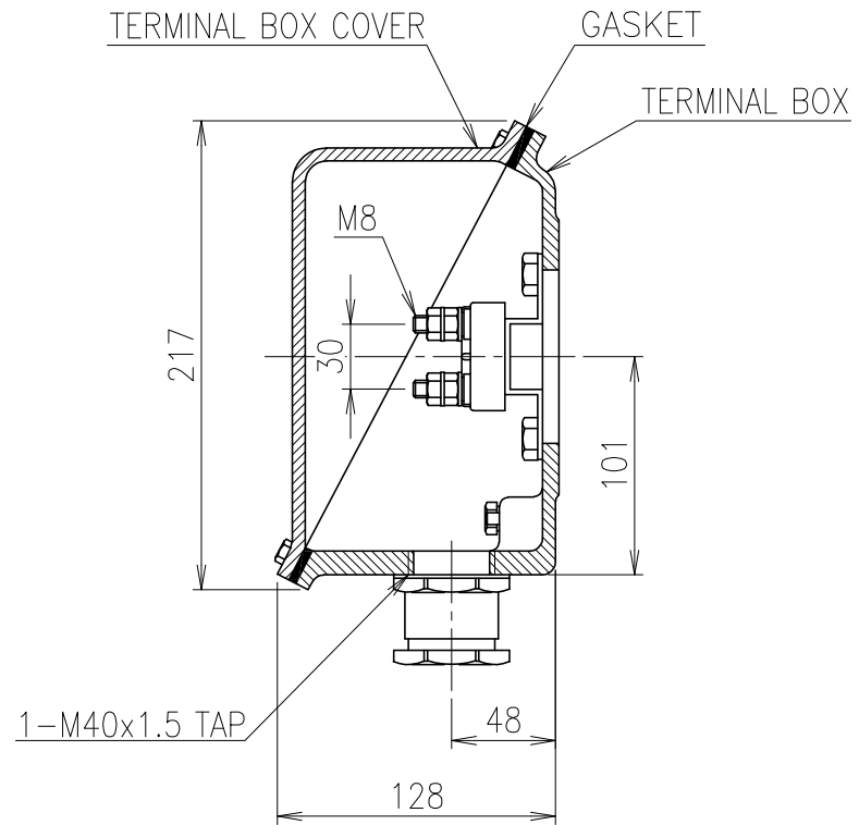
SEC. A-A'
